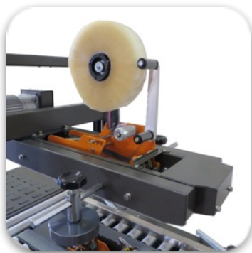
Offset Tape Head Design With Adjustable Box Side Guides.
